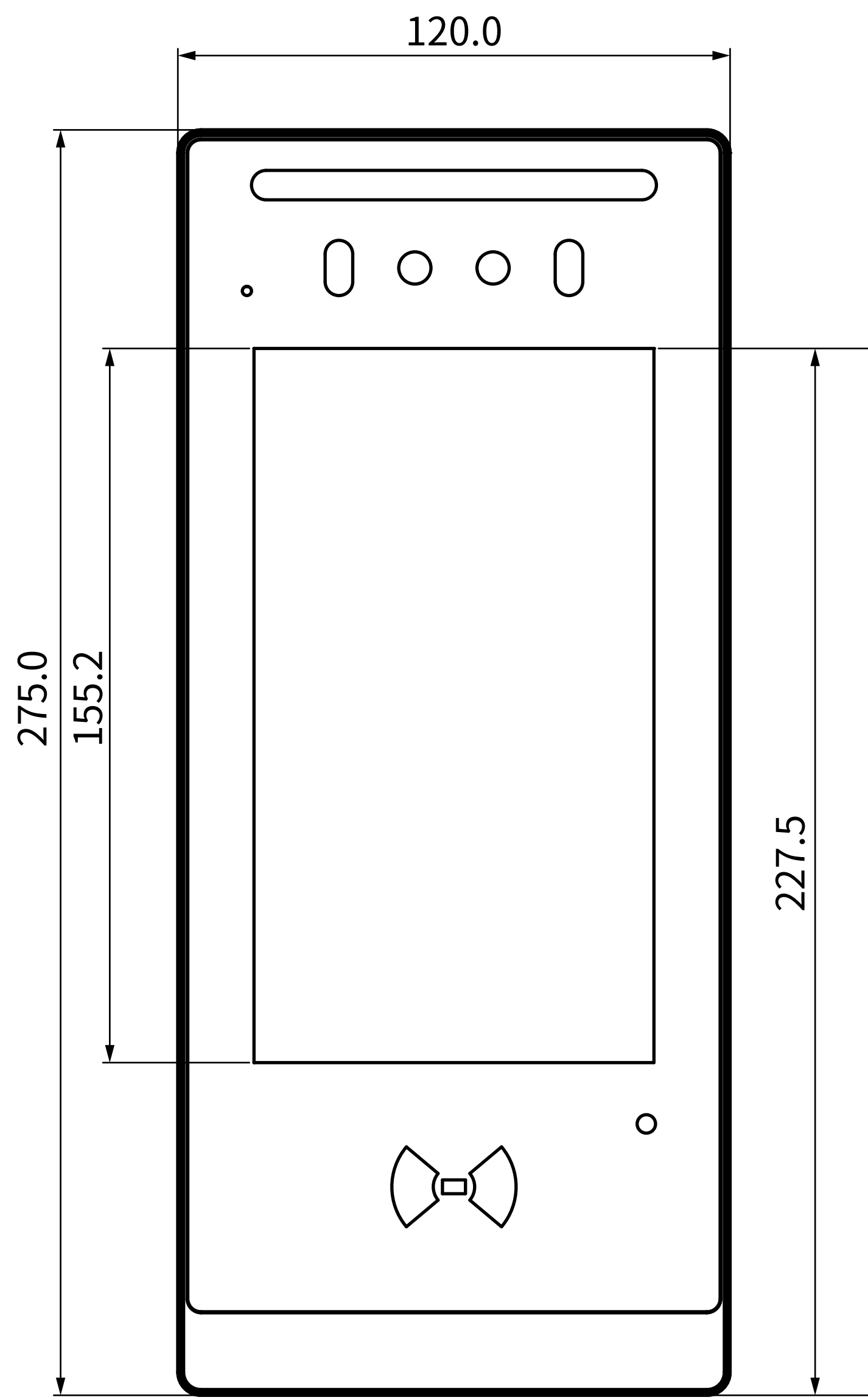
1 FRONT VIEW
