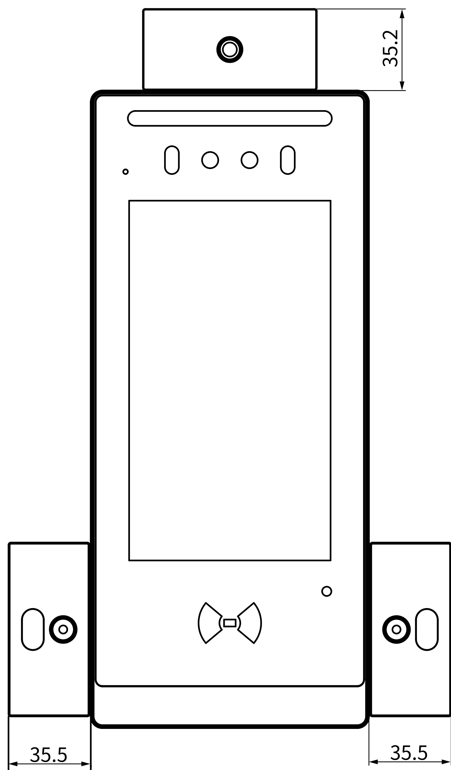
1 INTERCOM PANEL FRONT VIEW
