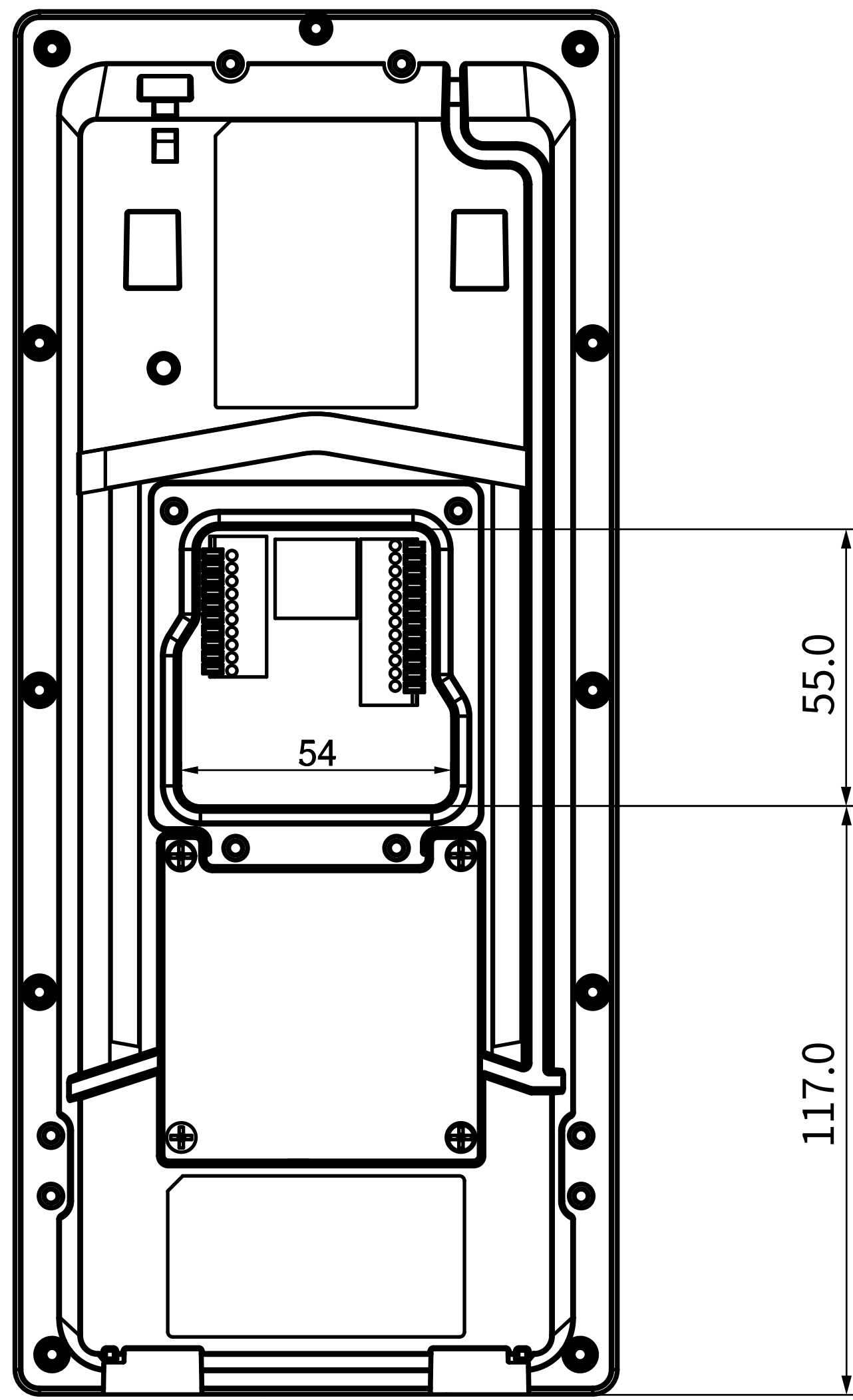
4 BACK VIEW
