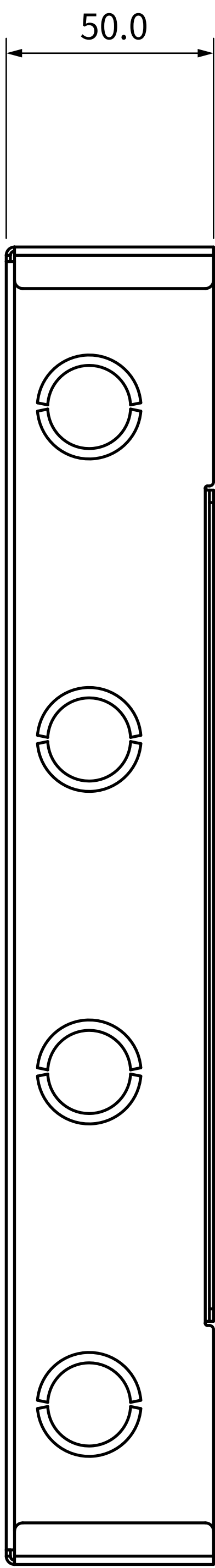
3 LEFT VIEW
