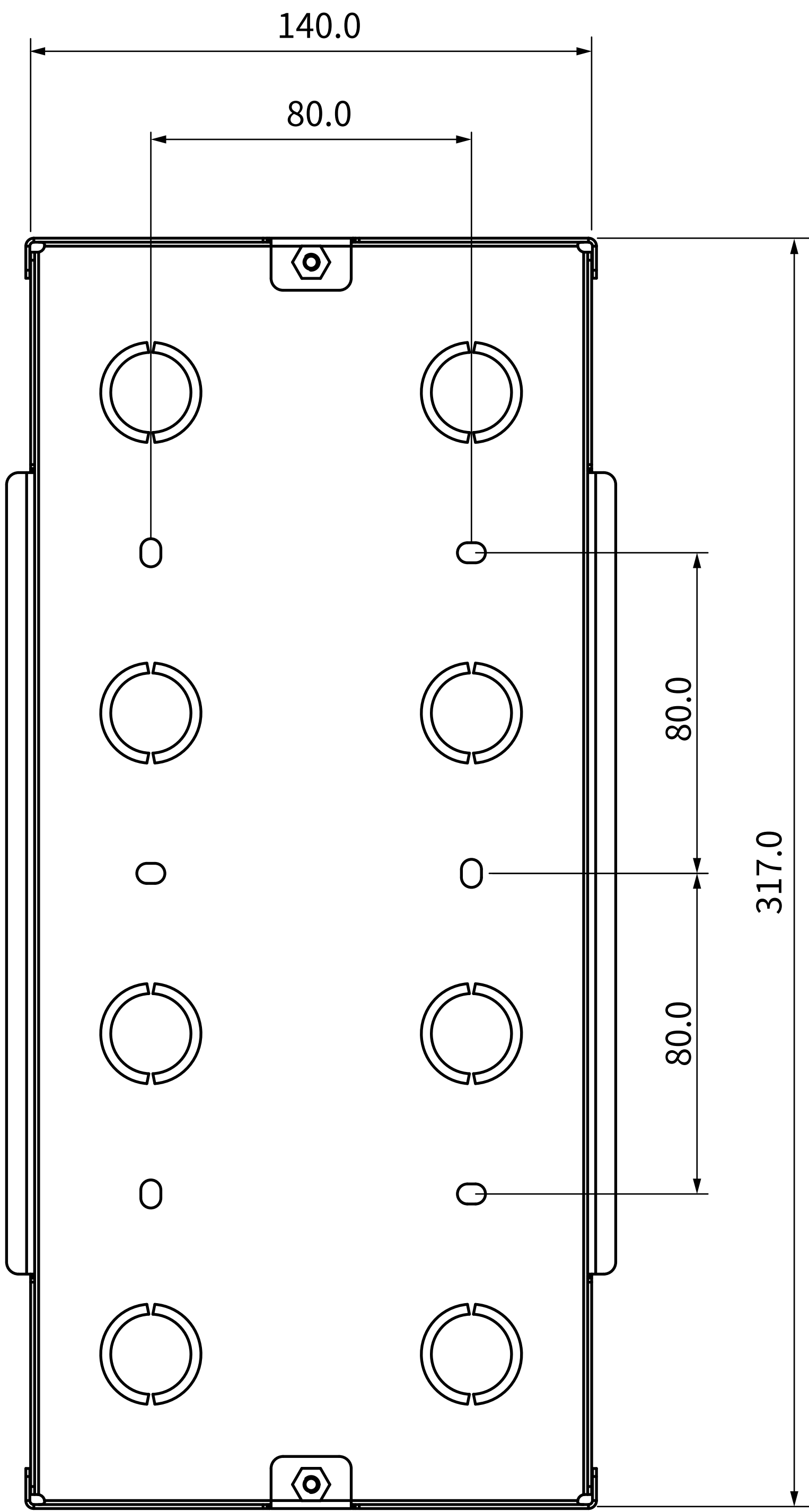
1 FRONT VIEW
