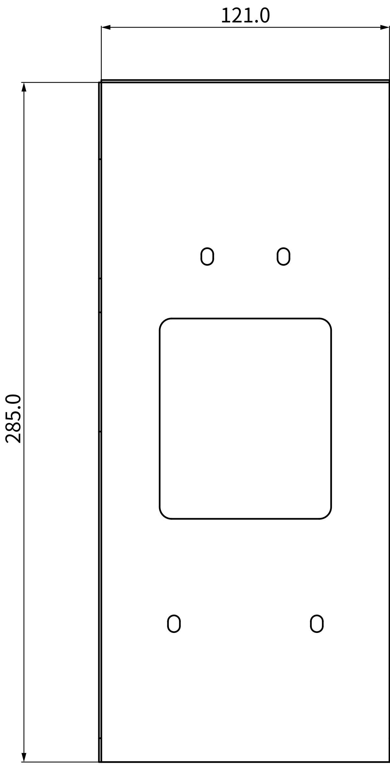
1 FRONT VIEW
