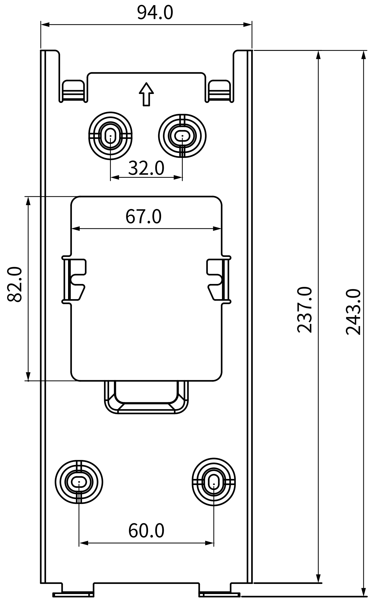
1 FRONT VIEW
