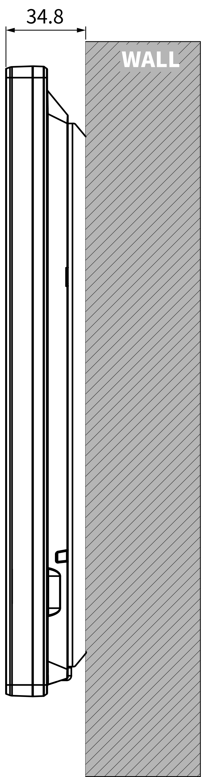
4 SIDE VIEW:INTERCOM ON WALL
